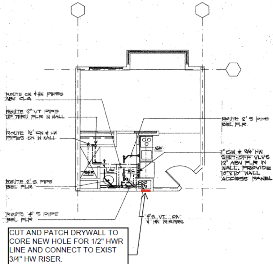
8 UNIT A1 DETAIL PLUMBING PLAN SCALE: 1/4" = 1'-0"
